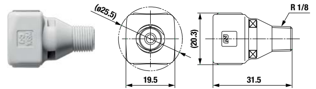
Dimensions (mm)
